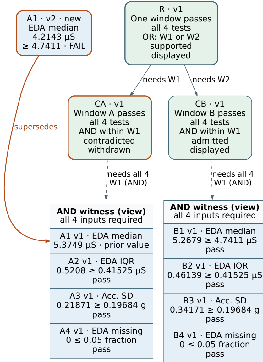
Fig. 3. Actual Neo4j generated-program view, PPG-DaLiA S1 episode 0, knowledge time 2331.01 s; requested and realized depth 2. This is the smallest complete eligible graph, with ID tie-breaking, among 87 programs. Windows A/B span 2270–2300/2150–2270 s. A1’s correction invalidates CA; CB still supports R. W1/W2 are alternatives at R; each route requires all four inputs. Blue rows are stored feature records. Dashed bundles summarize four DEPENDS_ON edges; AND enclosures are rendering constructs with exported row/edge mappings. Solid needs arrows are stored parent dependencies. Observation provenance is expandable; administrative details remain inspectable.
