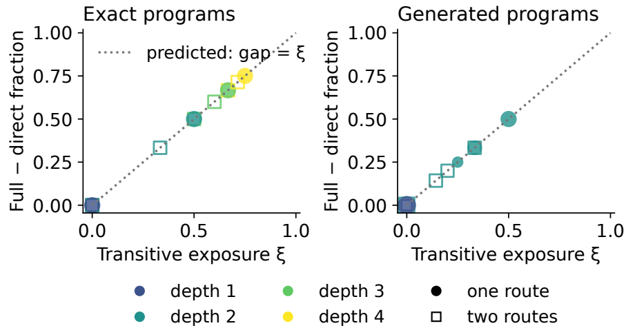
Fig. 5. Population-level structural test. Full-minus-direct correction fraction versus independently computed transitive exposure, separately for exact compiled and admitted GPU-generated programs. Points aggregate equal exposure, support regime and realized depth; size reflects batch count. The diagonal is the conditional prediction. This reports primary admission; the text gives the separate normalization sensitivity result.
