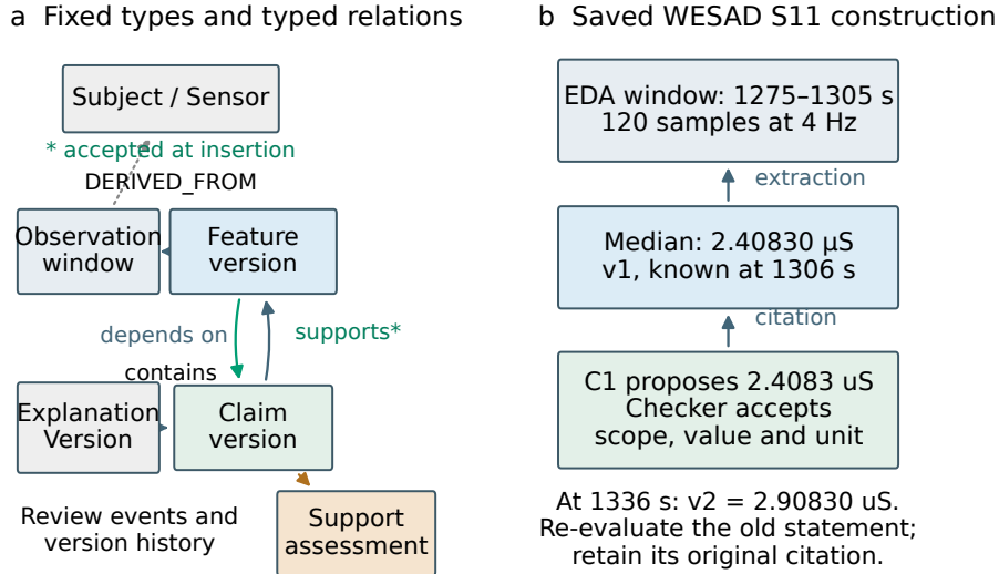
Fig. 1. Fixed vocabulary and actual instantiation. Blue denotes deterministic recording/feature construction, green a checked model proposition, grey identity or display administration, and amber assessment/version effects. The concrete path comes from the exported WESAD S11 correction scope; its source hash, sample indices and full IDs accompany the figure. Arrows have the stored direction. The displayed schema is a readable subset of the complete construction table.
