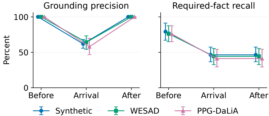
Fig. 4. Independent grounding precision and required recall for the same prior M1 answers at three discrete checkpoints, with subject-cluster 95% intervals. Each source has 160 transitions from 20 episodes and ten subjects across the four variants. No smooth recovery curve is inferred. Emitted-claim and required-fact denominators are given in the text; fresh-answer scores remain in Table 3.
