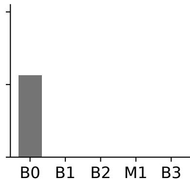
PPG-DaLiA
