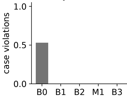
Synthetic
