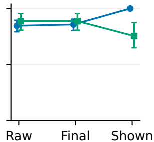
PPG-DaLiA
