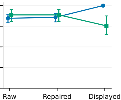
PPG-DaLiA
