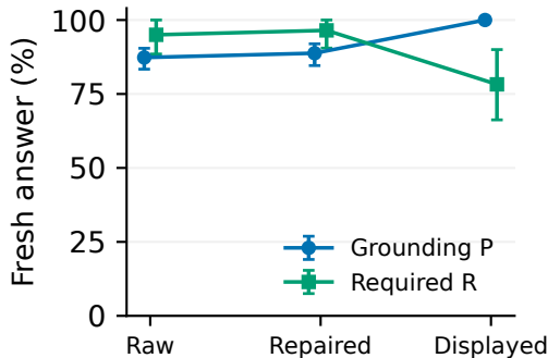
Synthetic
