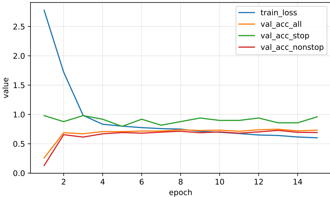
Two-opt policy learning curve
