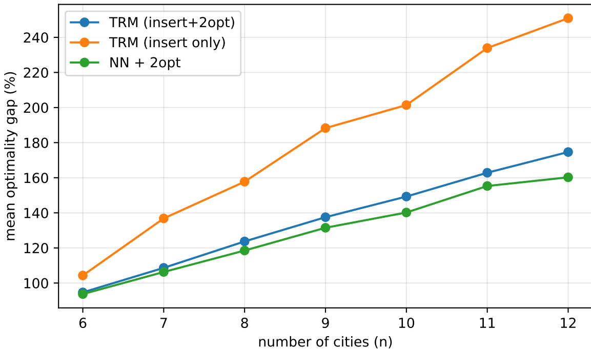
Scaling with n (exact optimum reference)
