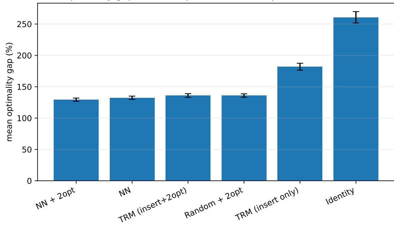
Optimality gap vs exact optimum (Held-Karp), mean \pm 95% CI
