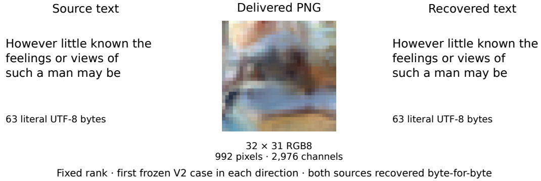
Figure 1: Actual artifacts selected by manifest order. A transports a canonical 16 \times 16 grayscale array through a verbatim, incomplete excerpt of its 616-token UTF-8 carrier, recovering all 256 pixels rather than an arbitrary image file. B shows complete 63-byte source/recovered texts and the actual 32 \times 31 RGB PNG. Pixels use nearest-neighbor enlargement. Each fresh receiver uses carrier, profile, shared context and key. The PNG row is withheld and prepended internally. Source equality is evaluated separately. The figure’s full-file note denotes local author material, not a reviewer-access link.
