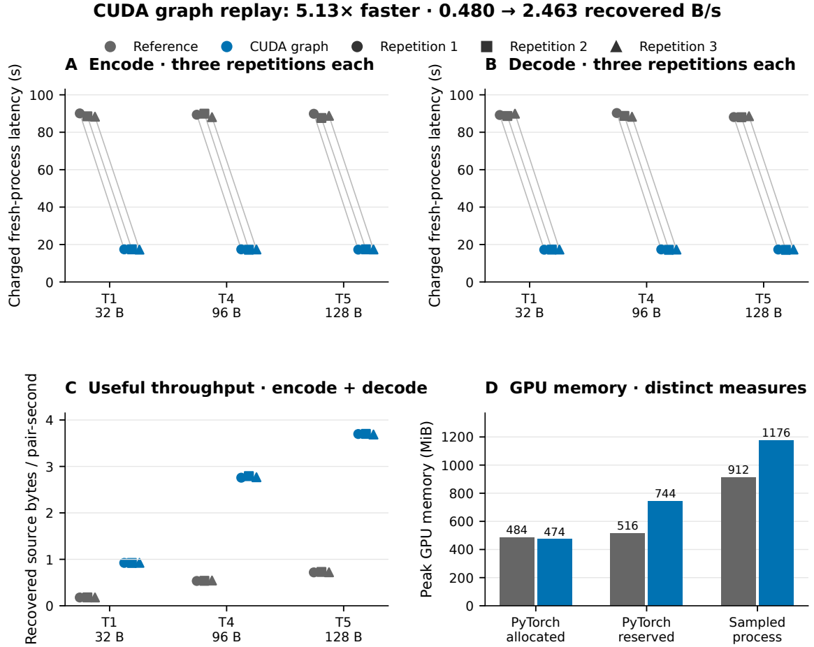
Figure 4: Development GPU benchmark on the pinned RTX 5000 Ada configuration. Fixed rank has three alternating-order matched repetitions for each of three payloads, not nine independent scientific payloads. Encode/decode latency includes fresh-process loading, graph setup and teardown. Throughput counts recovered source bytes over both processes. All 11 comparisons, including the additional single-payload gated/A1 checks, preserve exact probability streams, PNG bytes and recovery. Allocated, reserved and sampled process memory are overlapping measures and must not be summed.
