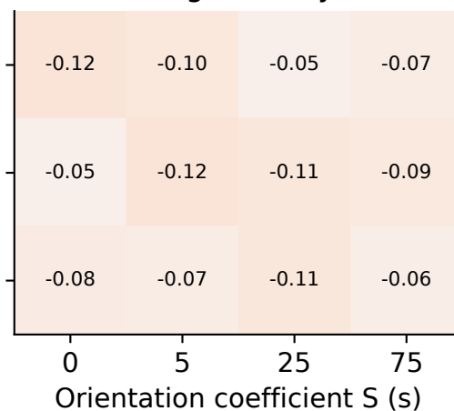
G minus Source-aware Q long memory
