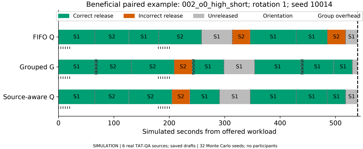
Figure 3: First individual run with more correct releases in G than FIFO Q. Orientation cost is zero. G releases one more correct answer, despite extra group overhead. The difference is which potential outcomes reach cutoff, not a saving in context reconstruction. This setting's cell mean actually favors FIFO.
