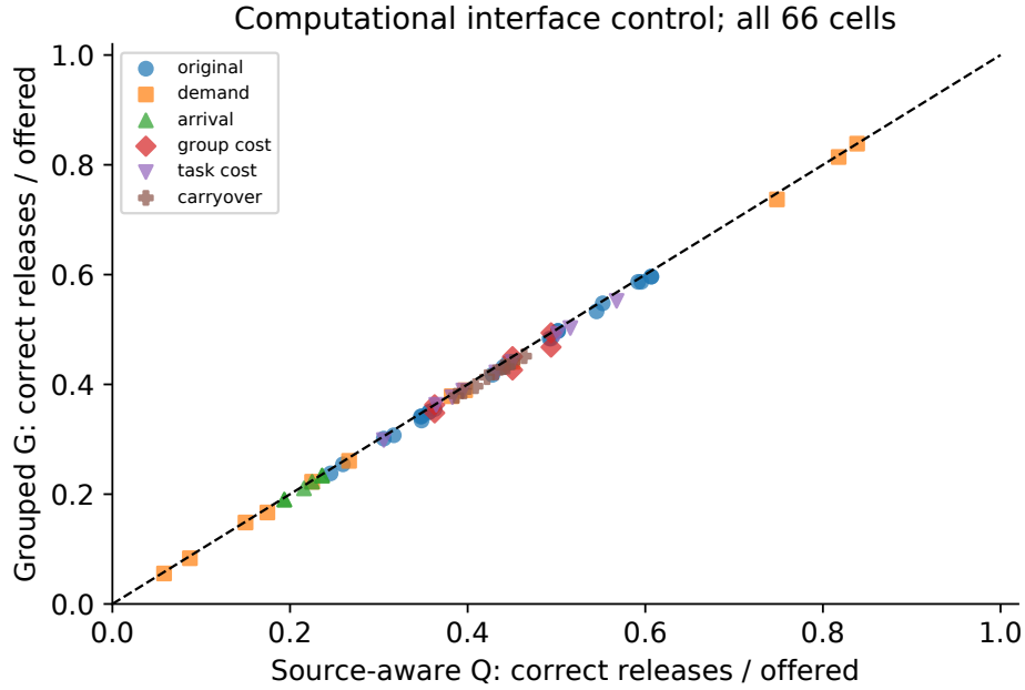
Figure 1: All 66 declared parameter-cell means. The diagonal is equal correct release fraction. No grouped mean exceeds the identically source-aware queue. Points reuse sources and parameter settings; they are not independent people or reports. Zero-overhead equality is structural.
