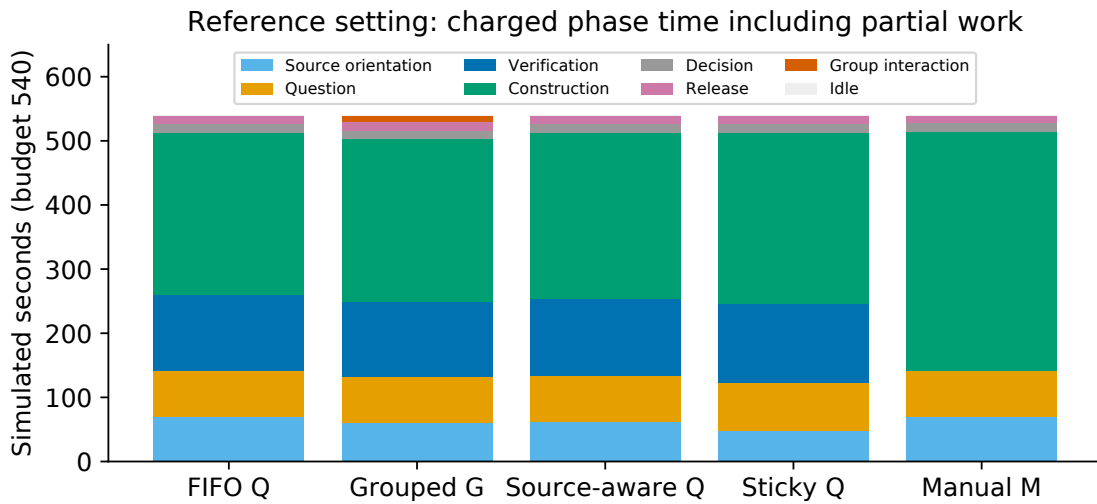
Figure 2: Assigned review phases in the original nine-minute reference setting. Partial last reviews consume time through cutoff. Components plus idle sum to 540 seconds. These are model components, not observed reading or attention time; the completed question subsets can differ.
