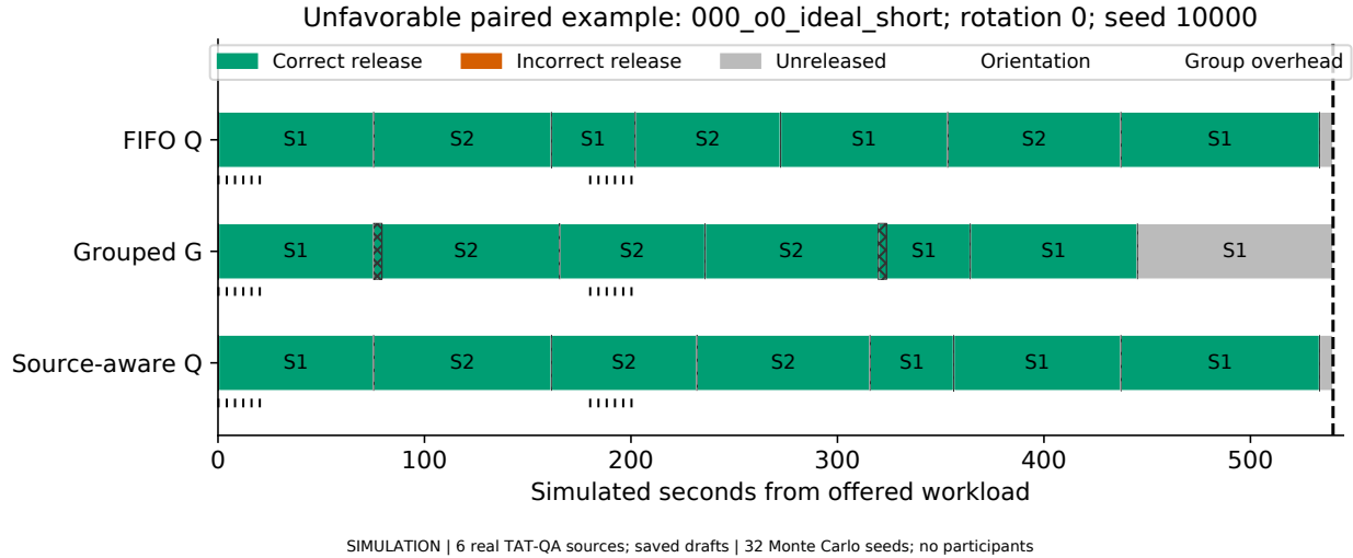
Figure 4: First adverse paired run. With zero orientation cost and ideal review, group overhead leaves a correct answer unreleased at cutoff that both queues release. Source grouping preserves the request but does not complete it. All subsequent approvals and repairs are simulated, not actual model continuations.
