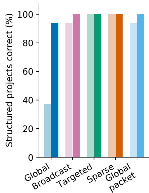
Strict / compatible parser
