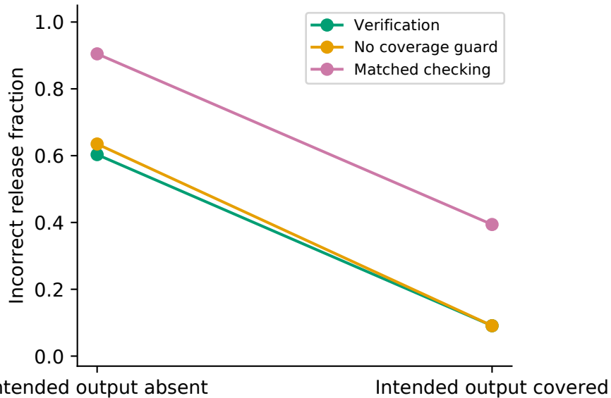
Generated-candidate diagnostic
