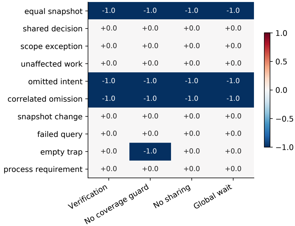
Synthetic: Answer difference (negative is fewer)
