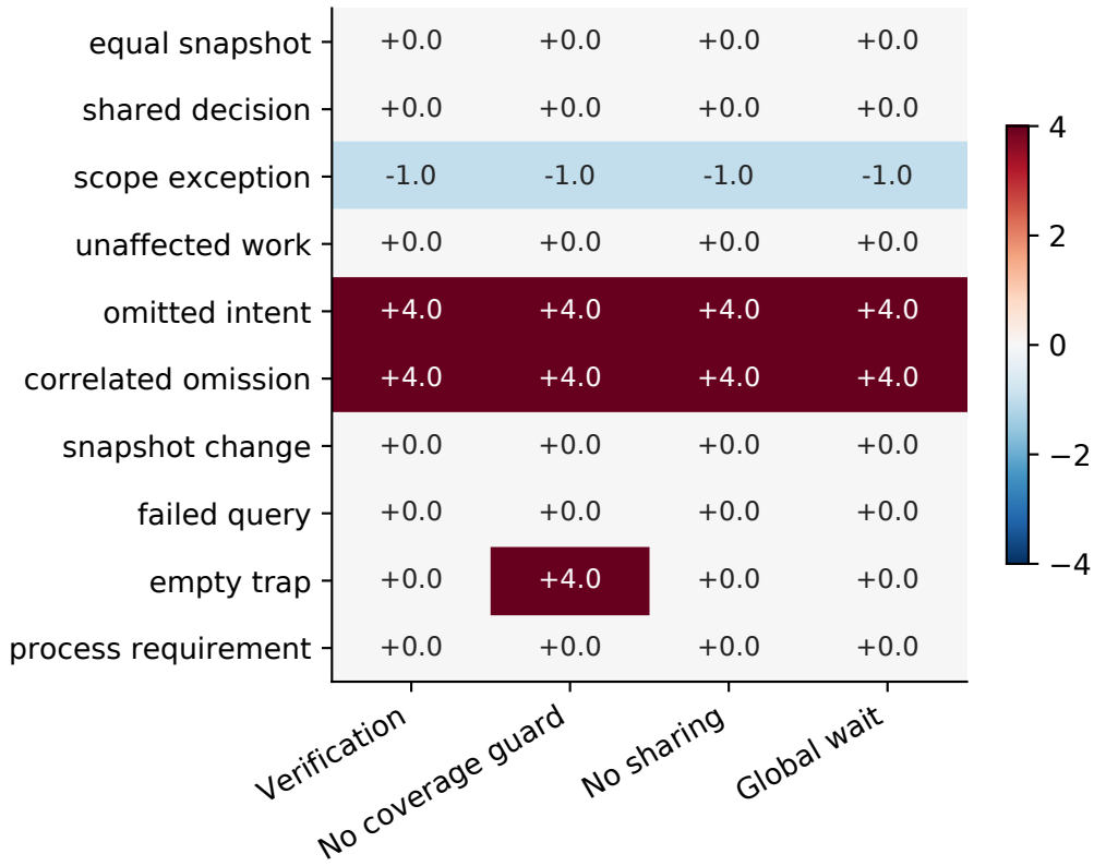
Synthetic: Loss difference (negative is better)
