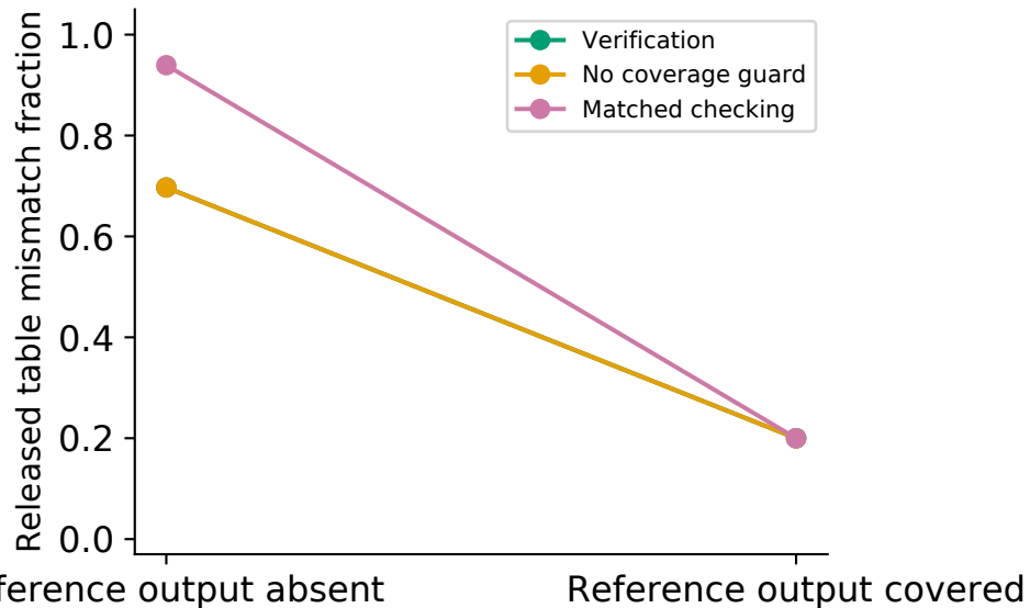
Generated-candidate diagnostic
