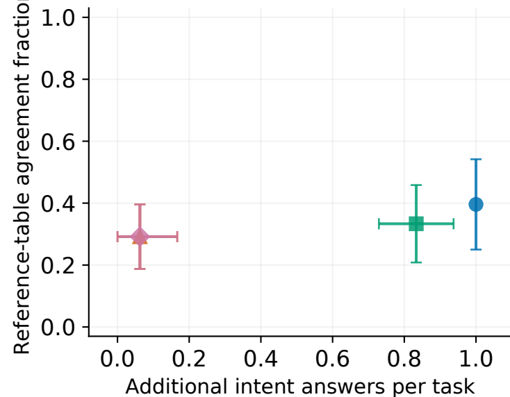
Generated candidates (24 databases)
