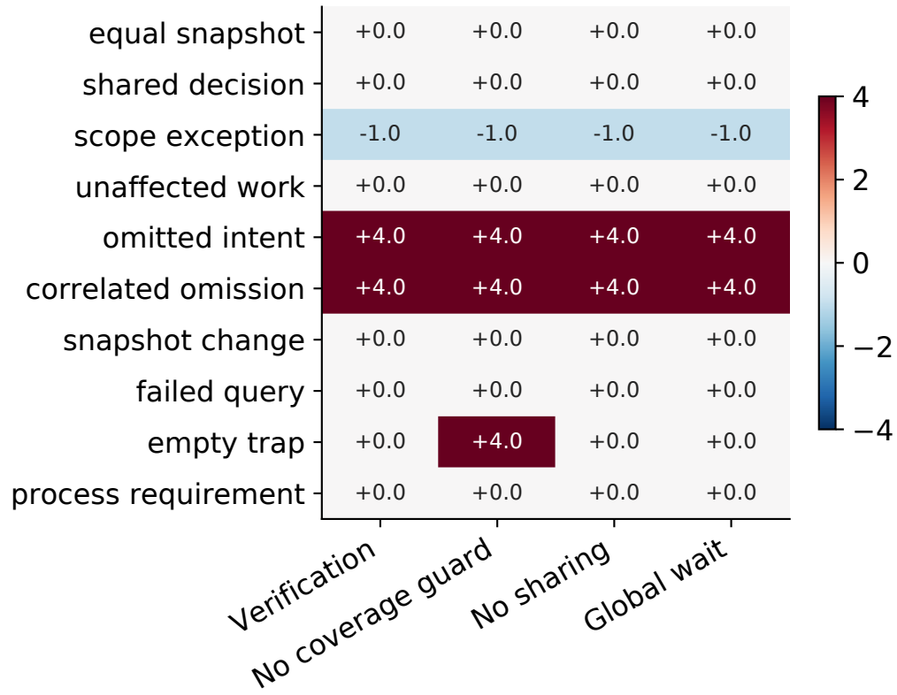
Synthetic: Loss difference (negative is better)
