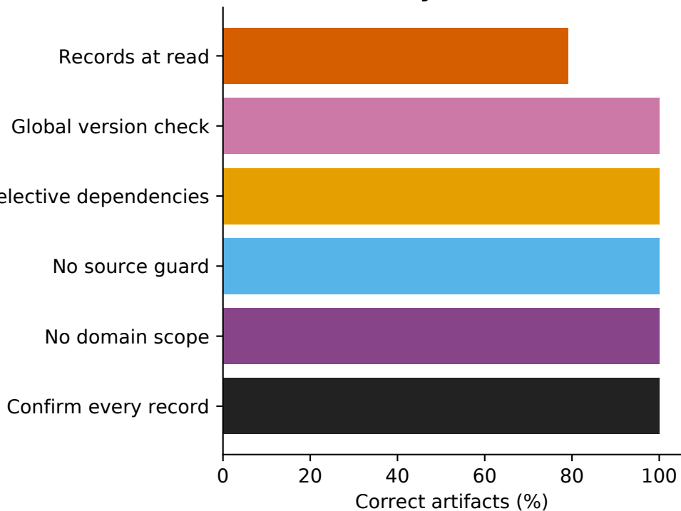
Quality ablations
