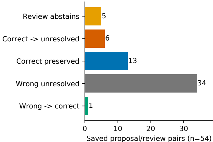
Generated reviewer transitions
