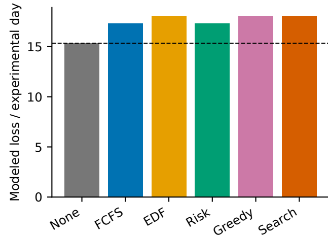
Secondary model-review allocation that ignores reviewer harm
