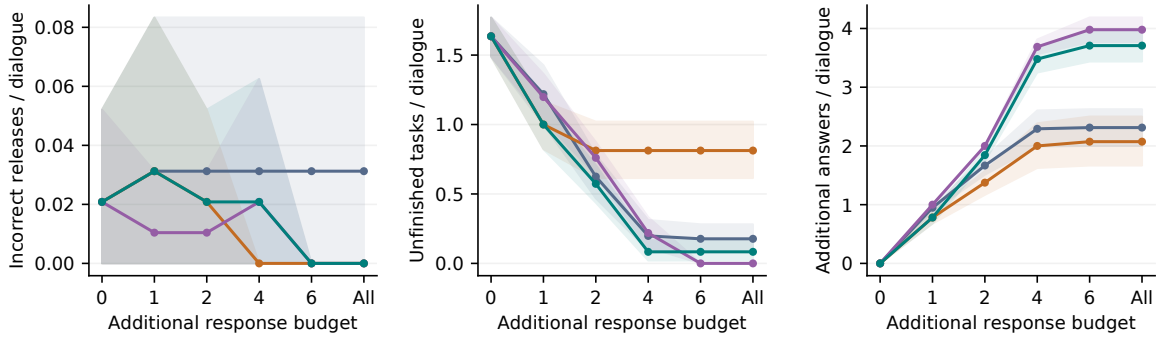
Figure 5: Empirical wrong and unfinished releases under simulated response budgets. These components remain separate from total loss. The task labels come from benchmark annotations and executable shortlist checks, not a human study.
