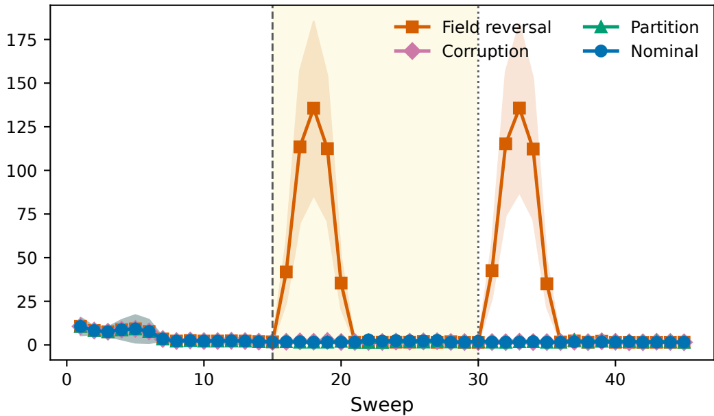
LOCO macrostate distance
