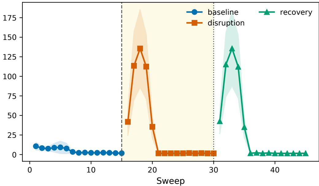
Macrostate distance
