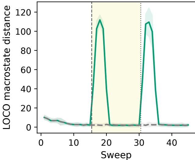
Qwen
