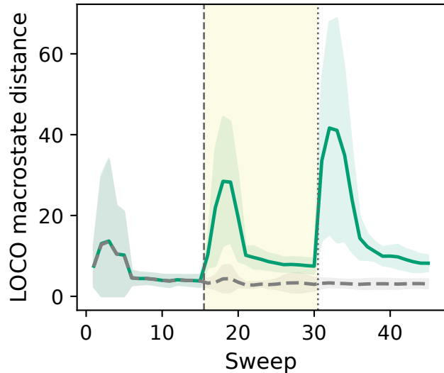
Granite
