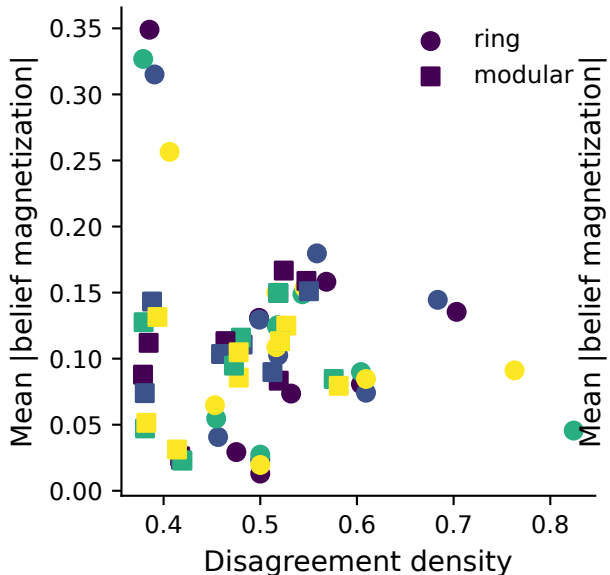
Collective finite-size regimes
