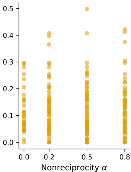
Belief susceptibility N\text{Var}(m_b)
