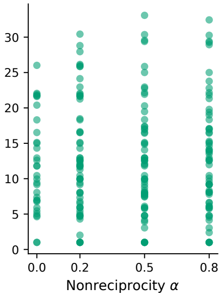
Correlation time (attempted updates)
