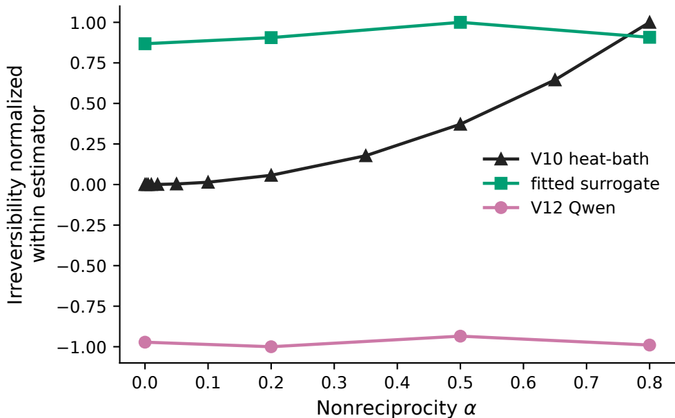
Normalized shapes; estimators are not numerically equivalent
