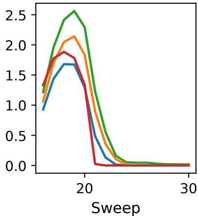
Configuration entropy
