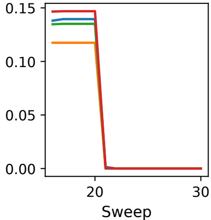
Susceptibility
