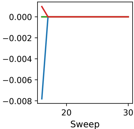
Belief magnetization
