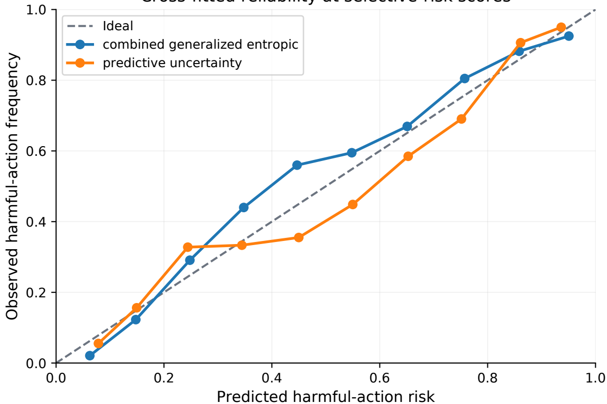
Cross-fitted reliability at selective-risk scores
