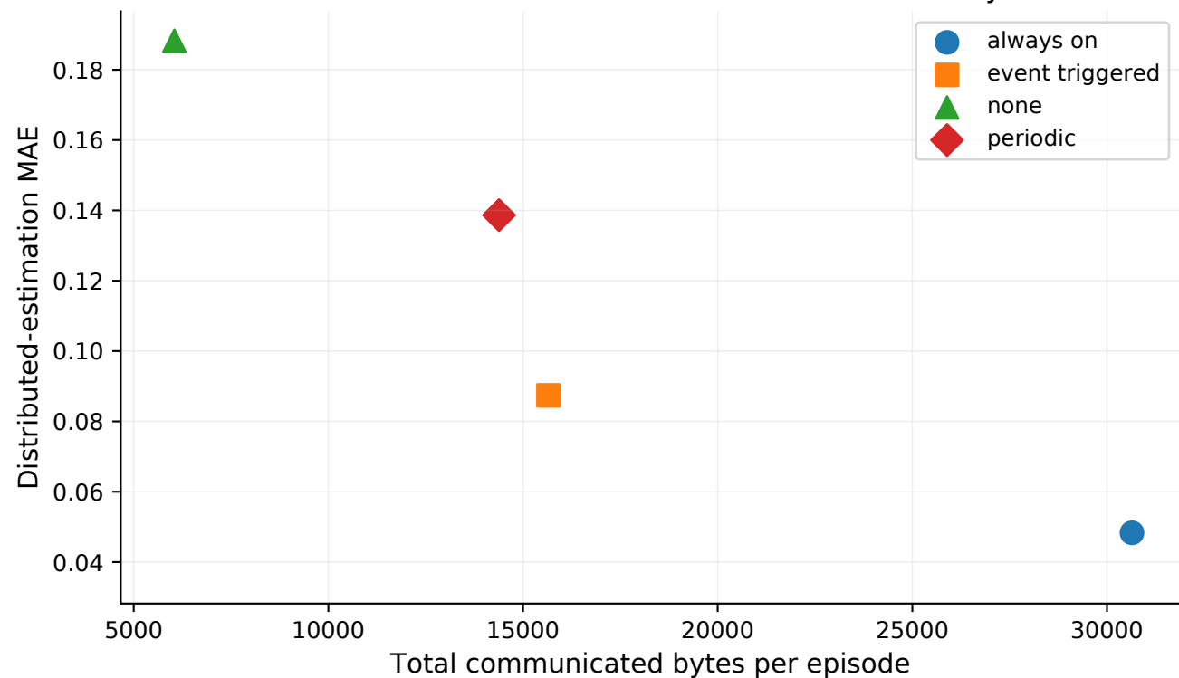
Communication cost versus consensus accuracy
