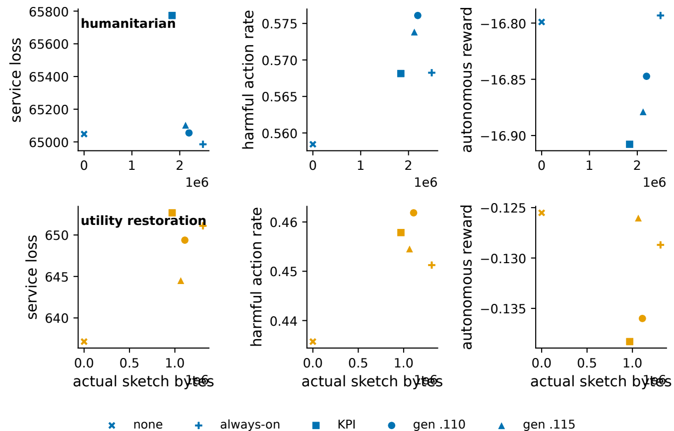
Deterministic-rule policy diagnostics (development pilot; n=6/application)
