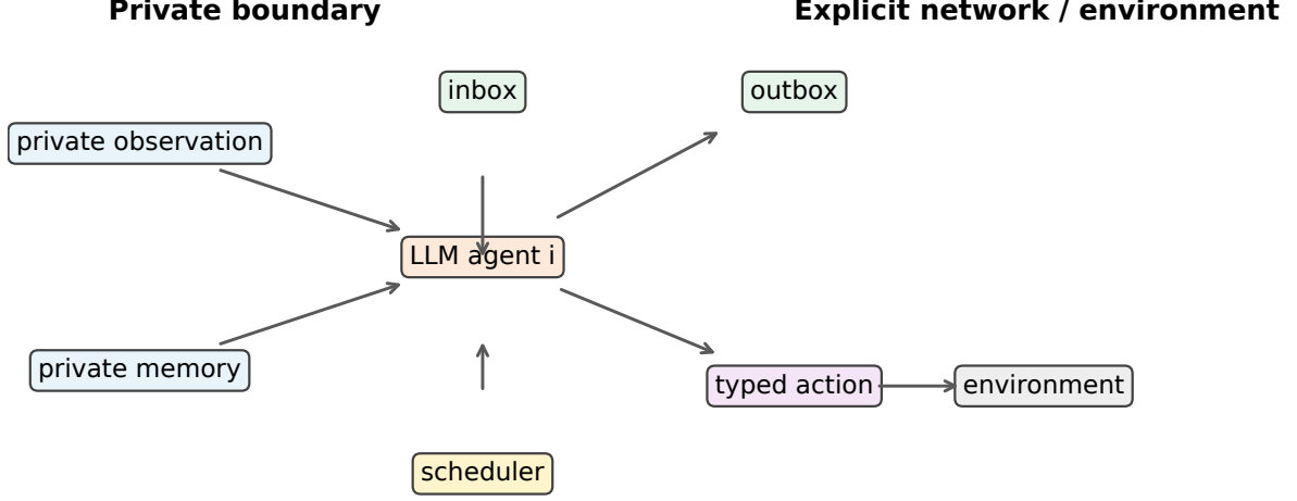
Figure 1: State-separated agent-instance information and authority boundary. The scheduler offers an update and transports the model-selected packet; it cannot inspect peer-private state or substitute a belief, action, commitment, memory, signal, or tool. The reduced state Z_t is evaluator-only.
