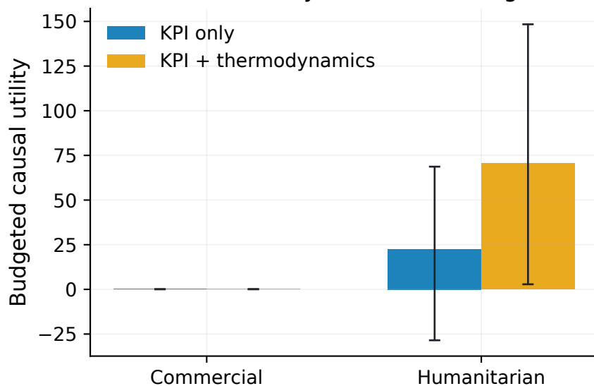
Absolute utility at matched budget
