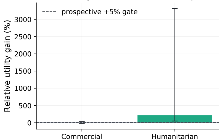
Relative gain with cluster bootstrap CI
