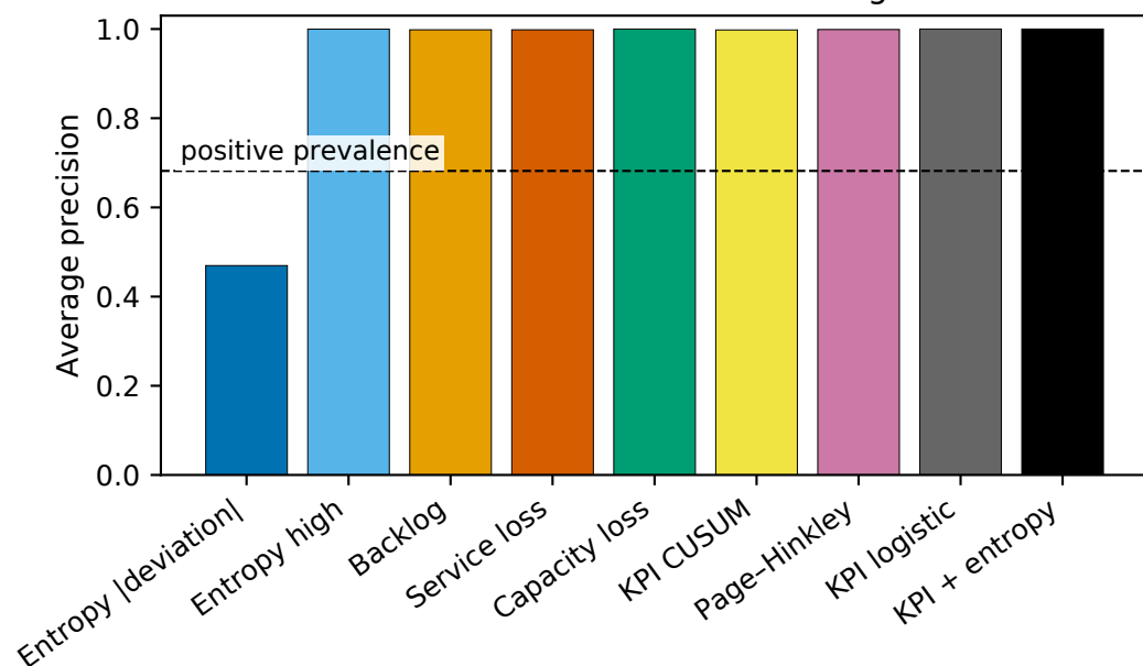
Humanitarian — seen holdout diagnostic
