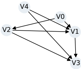
G0; mixture w=0.30
