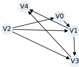
Component 2; w=0.70 representative
