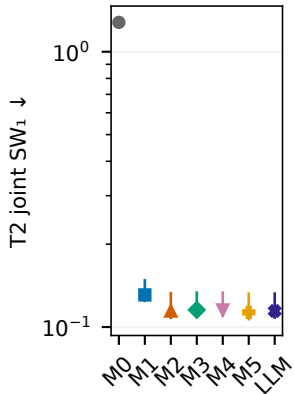
RGB: exploratory
