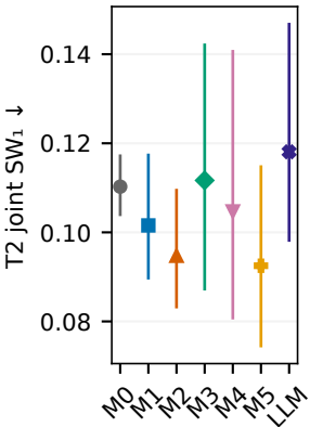
Semantic (5 SCMs)
