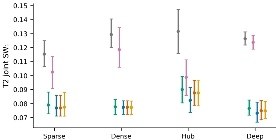
50-node heteroscedastic profiles
