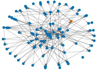
M5 component 1 w=0.989 representative
