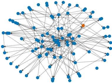
M5 component 2 w=0.011
