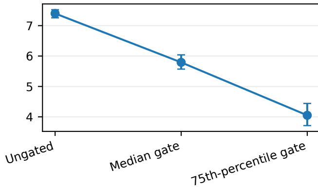
Visible-text exact recovery
