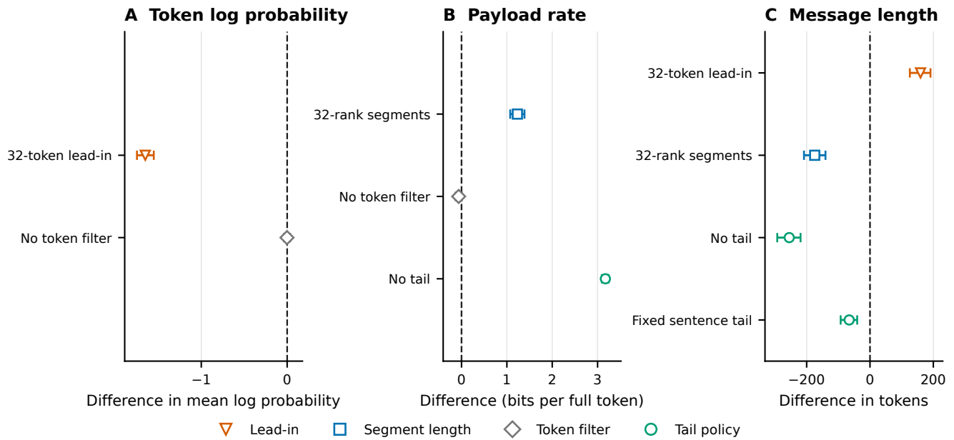
Figure S2. Complete ablation summary. Selected paired level-minus-canonical estimates are shown with payload-bootstrap 95% confidence intervals. Rows are exploratory/post-outcome evidence extraction from retained outputs. The Mistral roundtrip-stable-filter cell is unavailable for 48 work units; unavailable is not an execution failure. No-tail rate gains primarily reflect deletion of non-payload tokens and are not quality evidence.
