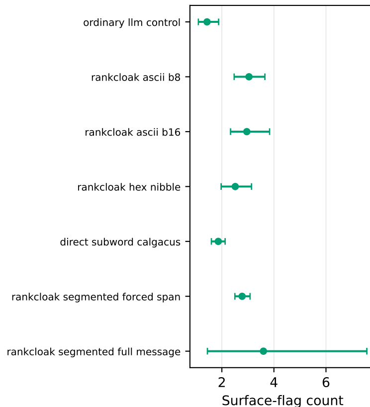
Automated surface diagnostics for the selected computational sample (95% prompt-template-cluster CIs; not human ratings)
