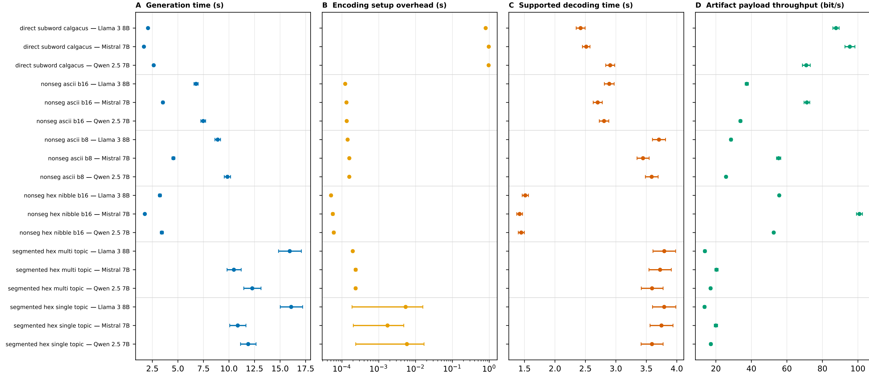
Primary-run computational timing and throughput (95% payload-cluster bootstrap confidence intervals)
