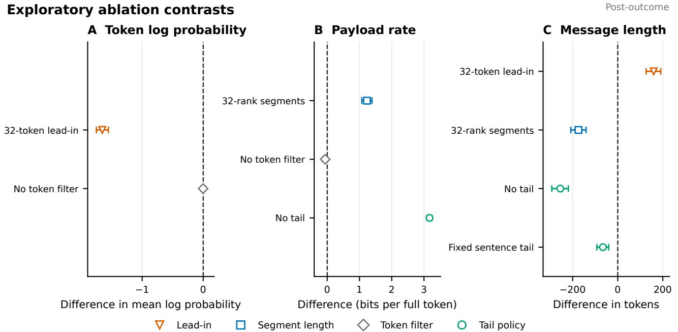
Figure S4. Ablation summary. Selected paired level-minus-canonical estimates are shown with payload-bootstrap 95% confidence intervals. Rows are exploratory/post-outcome evidence extraction from retained outputs. The Mistral roundtrip-stable-filter cell is unavailable for 48 work units; unavailable is not an execution failure. No-tail rate gains primarily reflect deletion of non-payload tokens and are not quality evidence.
