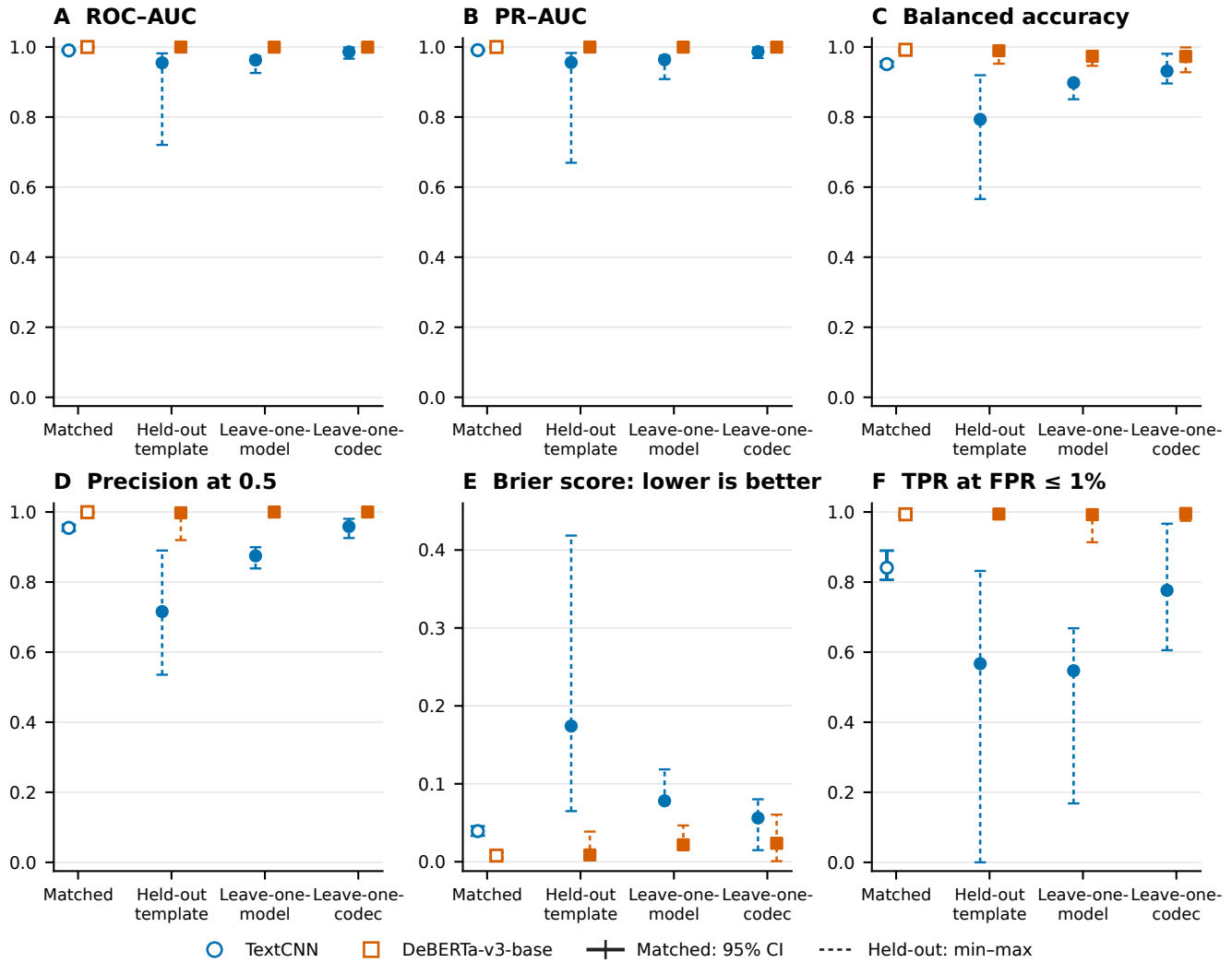
Figure S6. Full neural-detector evaluation. The six panels report confirmatory frozen endpoints together with supplementary exploratory metrics. Matched error bars are payload-group bootstrap 95% confidence intervals. Held-out regime bars span the minimum and maximum across prespecified splits and are not confidence intervals. Brier score is lower-is-better; high values in the other panels indicate stronger distinguishability and therefore weaker concealment.
