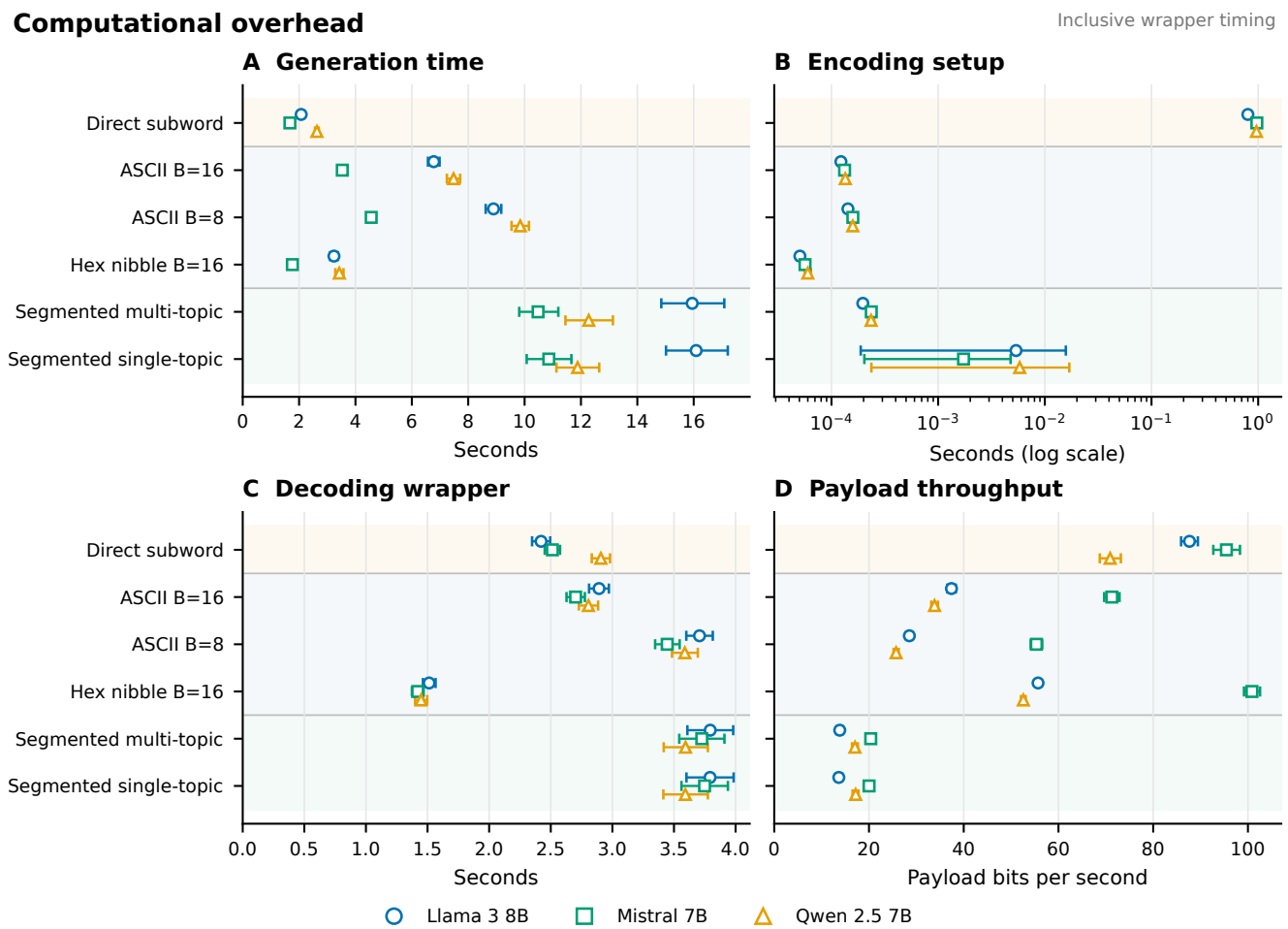
Figure S8. Complete computational-overhead summary. Primary model–protocol cells show payload-bootstrap summaries for inclusive generation, encoding setup, supported recovery, throughput, and effective rate. The setup panel uses a logarithmic axis because cells span several orders of magnitude. CPU time and repeated warm-up measurements were unavailable; wall time is not relabeled as CPU time.
