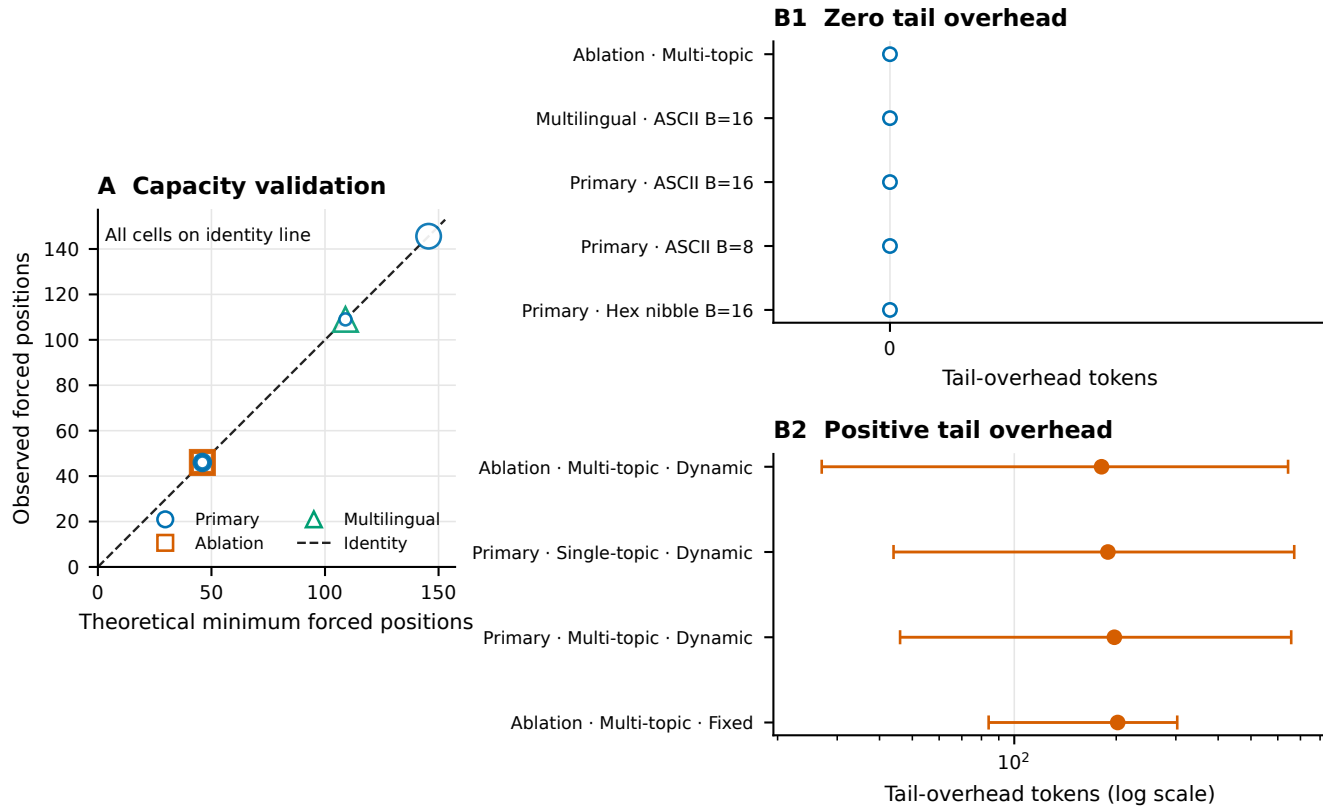
Figure S7. Theoretical capacity-tail validation. Fixed-radix payload length and effective full-message rate are checked against their declared algebraic bounds, while the cover-length residual isolates tokens beyond the forced payload positions. Across 17,424 retained records, 7,008 were evaluable for the complete plotted capacity and supported quality-bound checks; no forced-position, rate-bound, or evaluated quality-bound violation occurred. Positive residuals in 2,976 records represent natural tails or other cover overhead. This validation tests retained-field identities and differs from the empirical common-support frontier in Supplementary Fig. S3; neither analysis is evidence of human-perceived naturalness.
