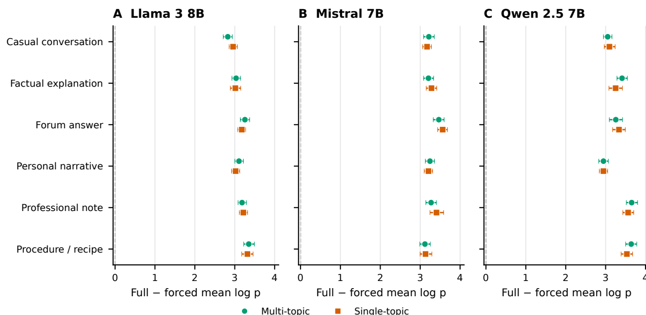
Figure S5. Exploratory tail gain by prompt category. Tail gain is full-message mean token log probability minus forced-span mean token log probability. The 8,280 paired segments arise from 1,440 segmented trials across three models, six prompt categories, and two topic schedules, yielding 36 displayed groups of 230 segments each. All group means are positive and range from +2.825721 to +3.652576. Uncertainty uses 2,000-resample payload-cluster bootstrapping stratified by payload class; independent payload-cluster counts are 40 for single-topic groups and 190 for multi-topic groups. This exploratory subgroup estimand is not the adjusted schedule contrast: adjusted source-quality contrasts range from -0.02214 to +0.01881, with Holm-adjusted p = 1.0 for all three models.
