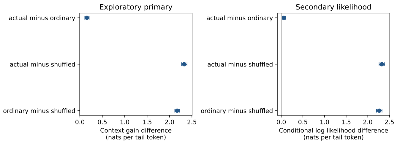
Figure S16. Paired boundary metric differences with payload-cluster 95% intervals. Context gain is the validated exploratory metric. Raw conditional likelihood is secondary. These automated results do not establish perceived naturalness.
