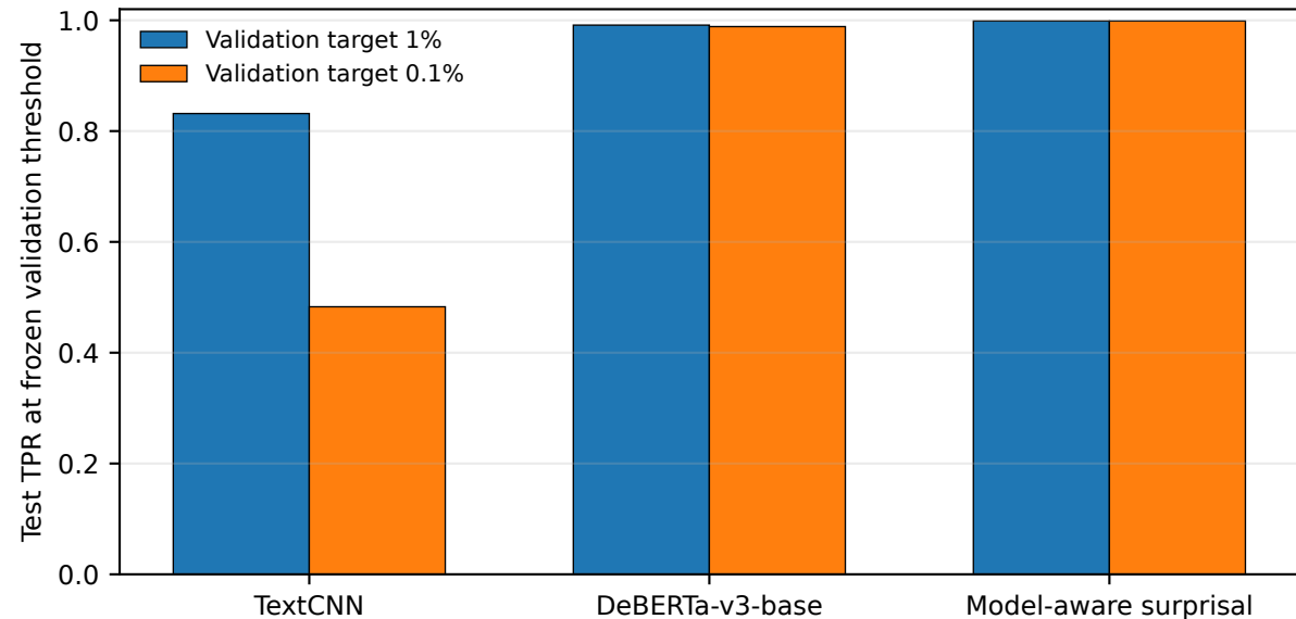
Matched-corpus low-FPR operating points
