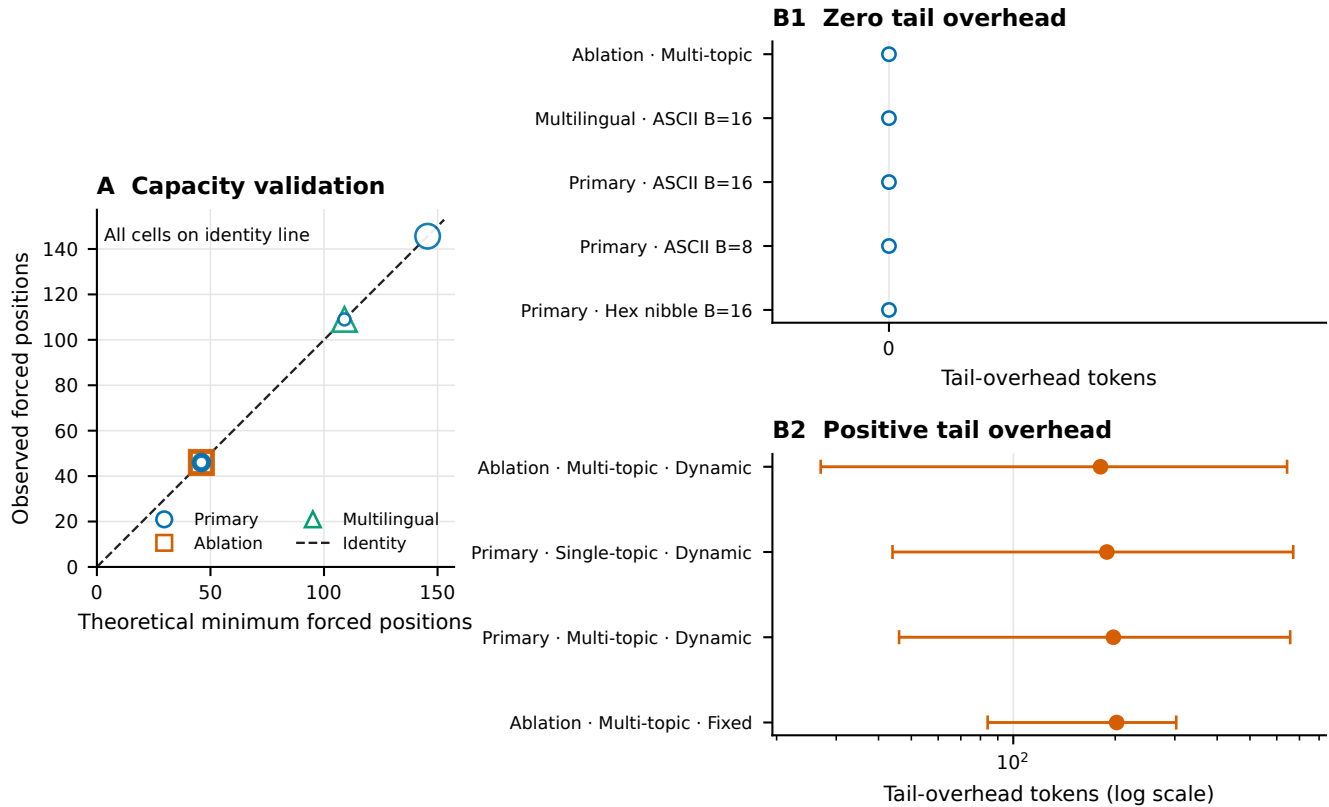
Figure S6. Theoretical capacity-tail validation. Fixed-radix payload length and effective full-message rate are checked against their declared algebraic bounds, while the cover-length residual isolates tokens beyond the forced payload positions. Across 17,424 retained records, 7,008 were evaluable for the complete plotted capacity and supported quality-bound checks; no forced-position, rate-bound, or evaluated quality-bound violation occurred. Positive residuals in 2,976 records represent natural tails or other cover overhead. This validation tests retained-field identities and differs from the empirical common-support frontier in Main Fig. 2; neither analysis is evidence of human-perceived naturalness.
