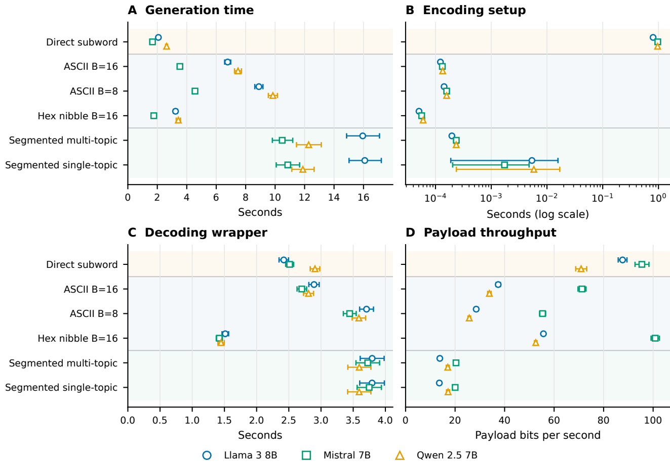
Figure S7. Complete computational-overhead summary. Primary model protocol cells show payload-bootstrap summaries for inclusive generation, encoding setup, supported recovery, throughput, and effective rate. The setup panel uses a logarithmic axis because cells span several orders of magnitude. CPU time and repeated warm-up measurements were unavailable and wall time is not relabeled as CPU time.
