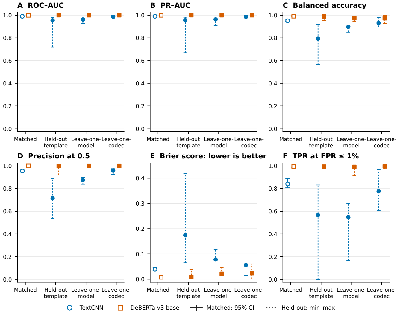
Figure S5. Historical V2 neural-detector evaluation. The six panels preserve the earlier frozen endpoints and supplementary exploratory metrics; current strictly deduplicated estimates are in Supplementary Note S12. Matched error bars are payload-group bootstrap 95% confidence intervals. Held-out regime bars span the minimum and maximum across prespecified splits and are not confidence intervals. Lower Brier scores are better; high values in the other panels indicate stronger distinguishability and therefore weaker concealment.
