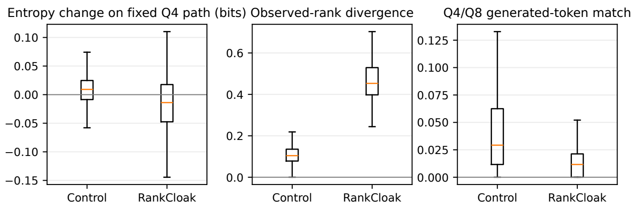
Figure S13. Matched quantization sensitivity. Same-path likelihood/rank comparisons and independently generated token-path agreement are paired within one pinned Qwen revision.
