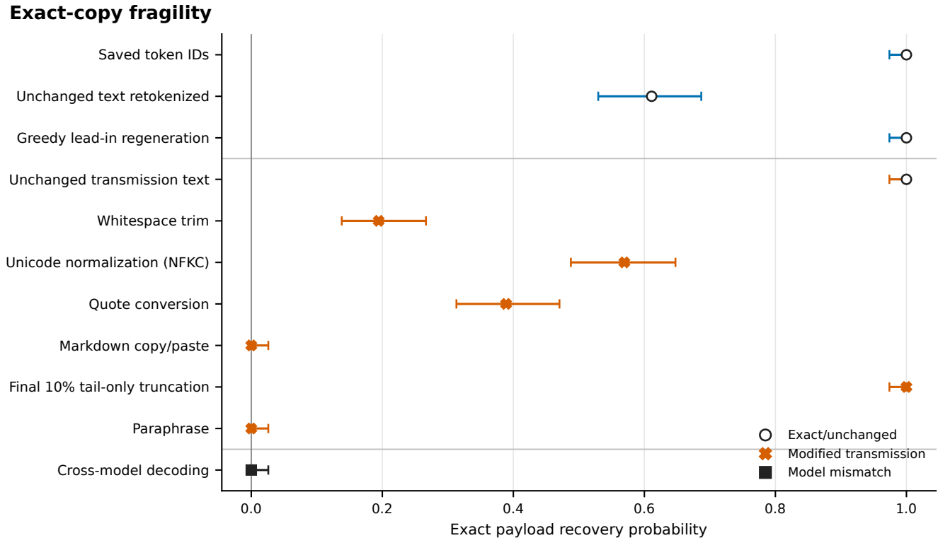
Figure 2. Exact-copy fragility. Recovery proportions and Wilson 95% intervals are shown for the principal replay and transmission conditions. Saved token IDs preserve the strongest replay contract; visible-text detokenization/retokenization already reduces recovery. NFKC normalization, quote conversion, and trimming reduce it further, while markdown copy/paste, paraphrase, and cross-model decoding yield no successful payloads. Final-10%-tail truncation removes only declared non-payload tail tokens and must not be interpreted as arbitrary truncation tolerance. The full transformation matrix, denominators, limited canonicalization cells, and first-divergence diagnostics appear in Supplementary Figure S1 and Supplementary Note S4.
