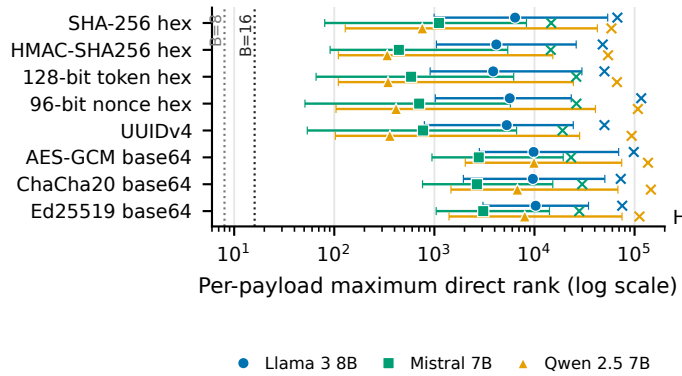
B Direct rank pressure
