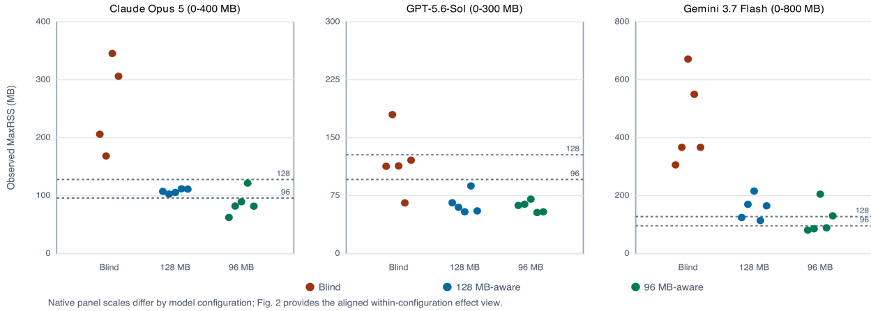
Figure A1. Every retained executable MaxRSS observation is shown in native MB. Each panel uses its own MB scale to reveal the within-configuration distributions; the panel heading states that scale. Dashed lines identify the 96 MB and 128 MB observed-RSS reference boundaries. Blind and 128 MB-aware results provide reference distributions; the 96 MB programs are independently sampled condition-level observations.
