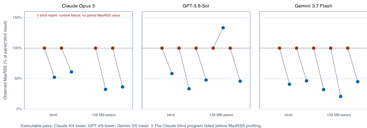
Figure 1. Each executable pair is indexed to its own blind MaxRSS result (blind = 100%). The figure preserves the one GPT higher-RSS outcome. Claude rep04_A failed under Python 3.9.6 before MaxRSS profiling and therefore has no pair-indexed value; the failure remains in the correctness denominator.
