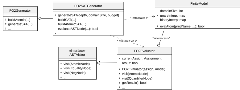
Figure 3.3: UML Class Diagram detailing the semantic SAT generation architecture. The FO2SATGenerator orchestrates the FiniteModel . It heavily relies on the Visitor Pattern via the FO2Evaluator to safely traverse the AST and compute semantic truth values without altering the underlying node structures.
