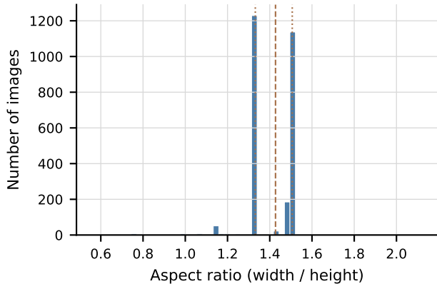
(b) Aspect ratio: median 1.427 [1.332, 1.507]
